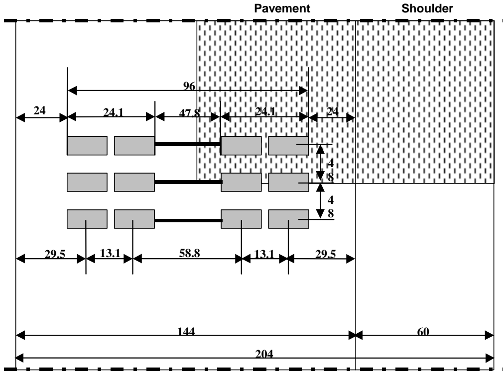
Figure 6.3 - Tridem Load Pattern
