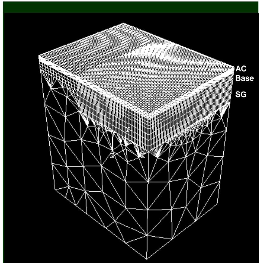
Figure 6.5 - Finite Element mesh for Pavement with 6-in. Thick AC Layer
