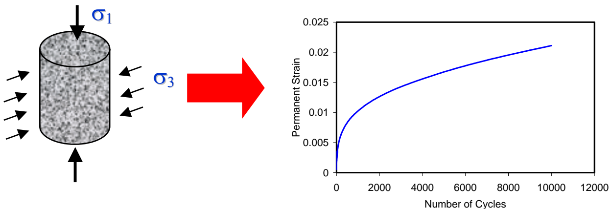
Figure 4.4 –Laboratory Tests to Obtain Parameters \alpha and \mu
