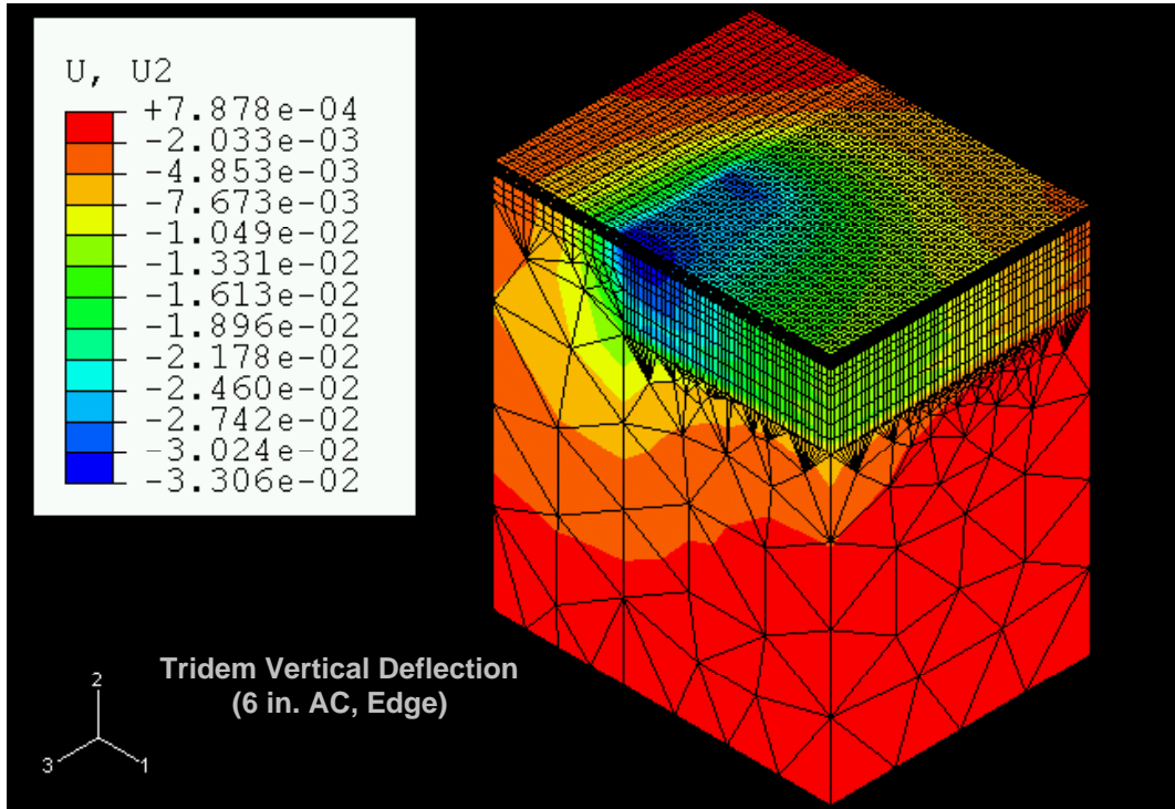
Figure 6.6 – Variation in Vertical Deflection under a Tridem Load Configuration
